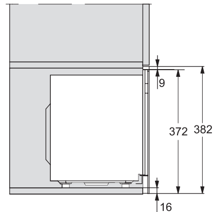
M223xSC, AB36, installation drawing
