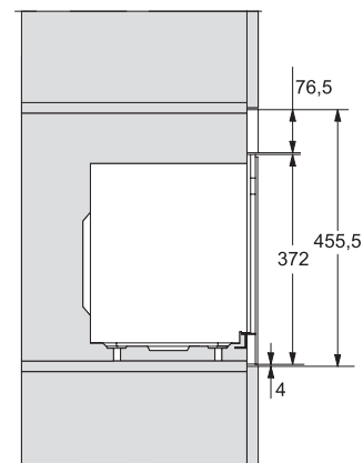
M223xSC, AB45-2, side view installation drawing
