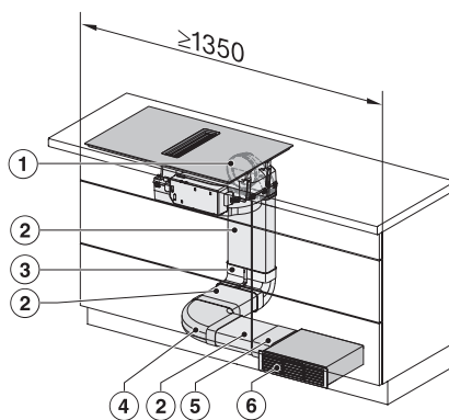
KMDA7676-1FL, KMDA7876-1FL, KMDA7676FL, KMDA7876FL – Installation variant 1 Basis
