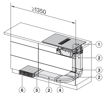
KMDA7676-1FL, KMDA7876-1FL, KMDA7676FL, KMDA7876FL – Installation variant 2 Basis
